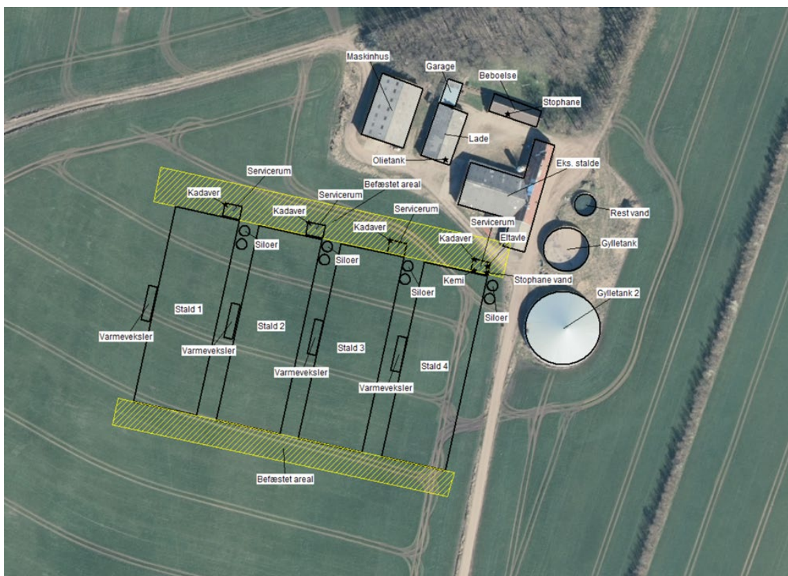
Figur 1. Situationsplan.
