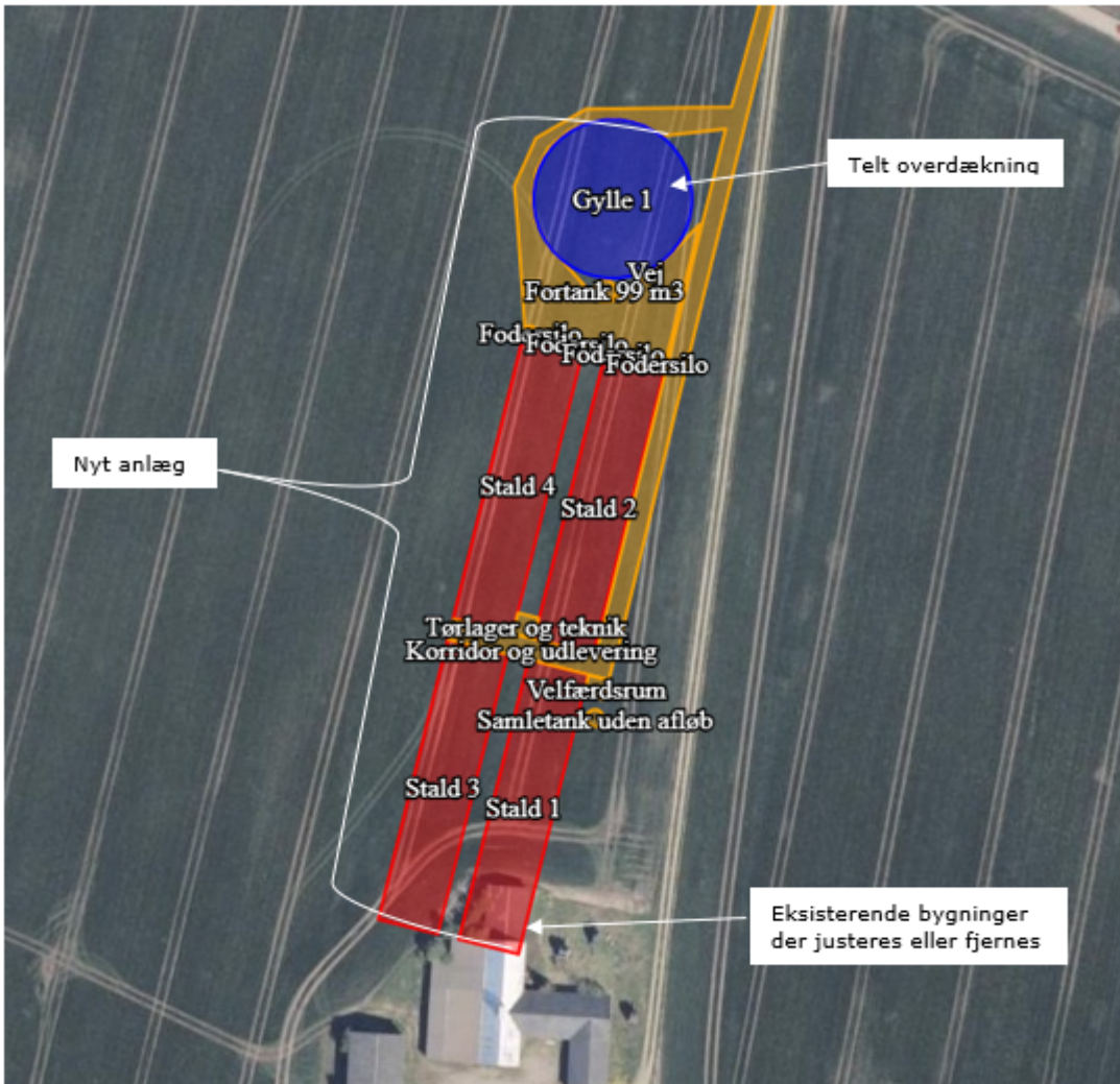
Figur 1. Situationsplan
